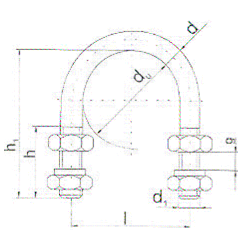
Pipe handles TYPE "E"
